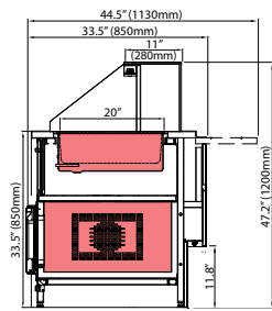
Bain Marie w/storage FRBME
