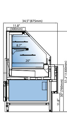
Grab 'n' Go w/storage FRSMVT
