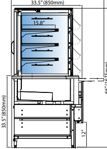
Multideck w/ Storage FRMDVS
