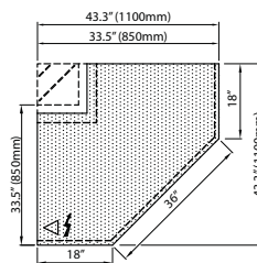
90° Interior Counter FRN-CI90
