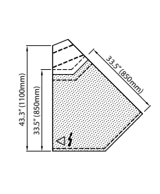
45° Interior Counter FRN-CI45
