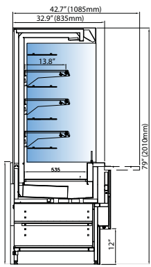
Open Multideck FRMR
