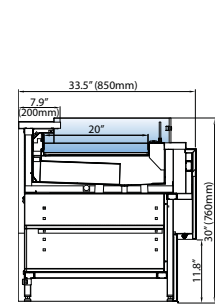
Grab 'n' Go low glass w/out storage, FRIS
