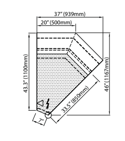
45° Exterior Counter FRN-CE45
