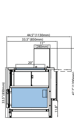
Refrigerated w/storage, FRTRT
