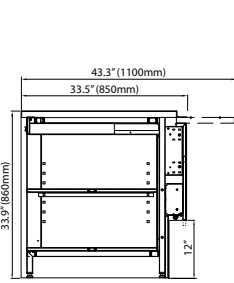
Neutral Counter FRN
