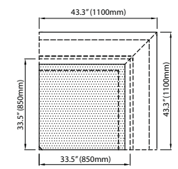
90° Exterior Counter FRN-CE90
