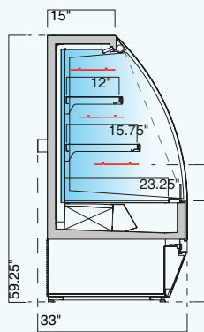
SMVCT 3N H15 3M2 ventilated
