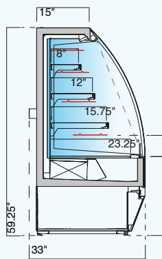
SMVCT 4N H15 3M2 ventilated
